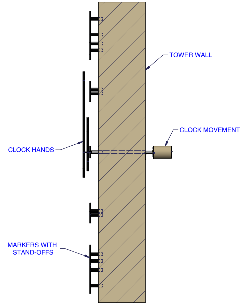
SECTION B-B
