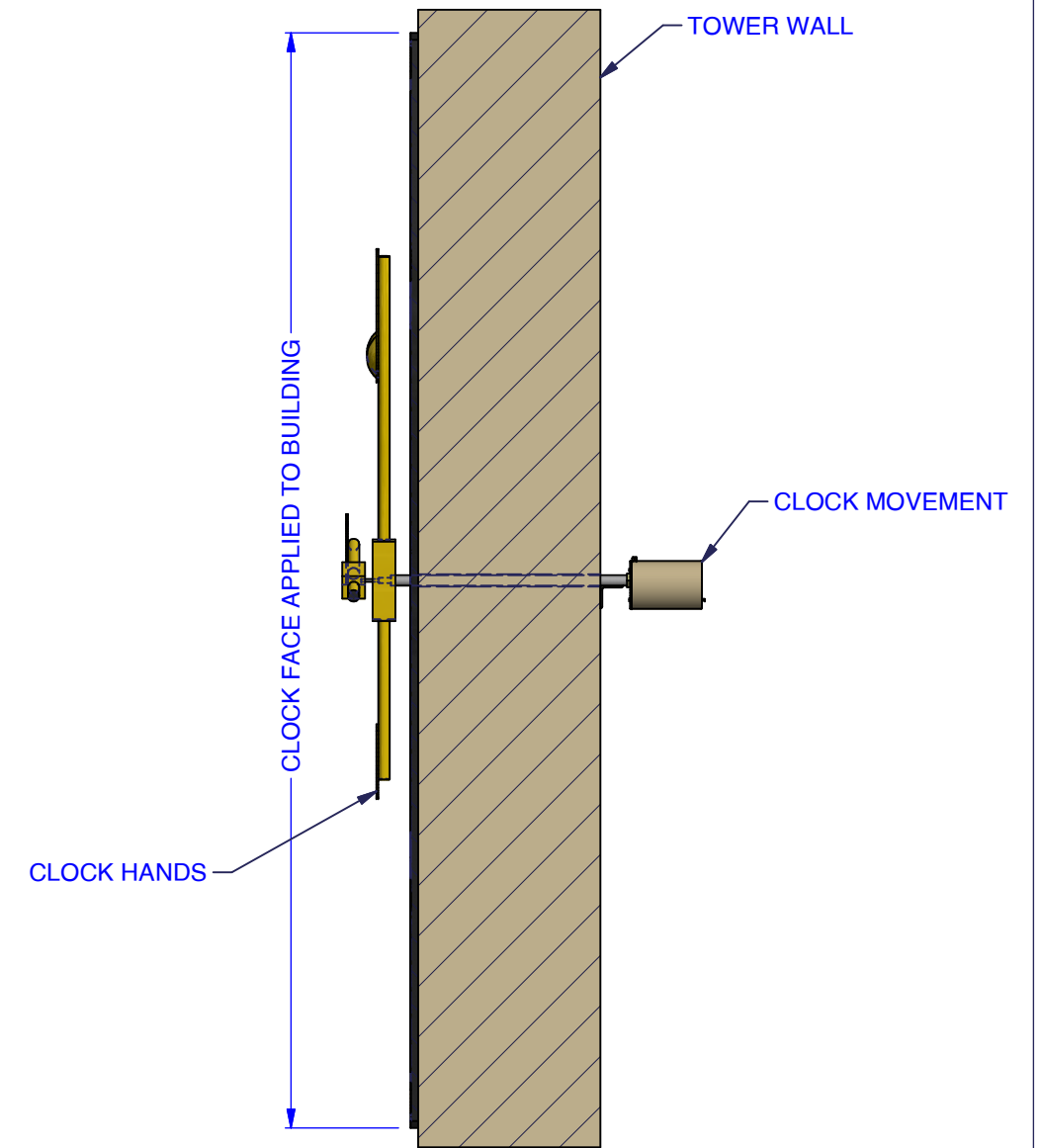
SECTION A-A SECTION THRU TOWER WALL
