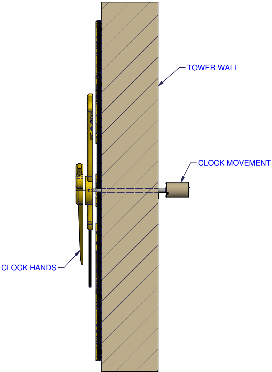
SECTION B-B
