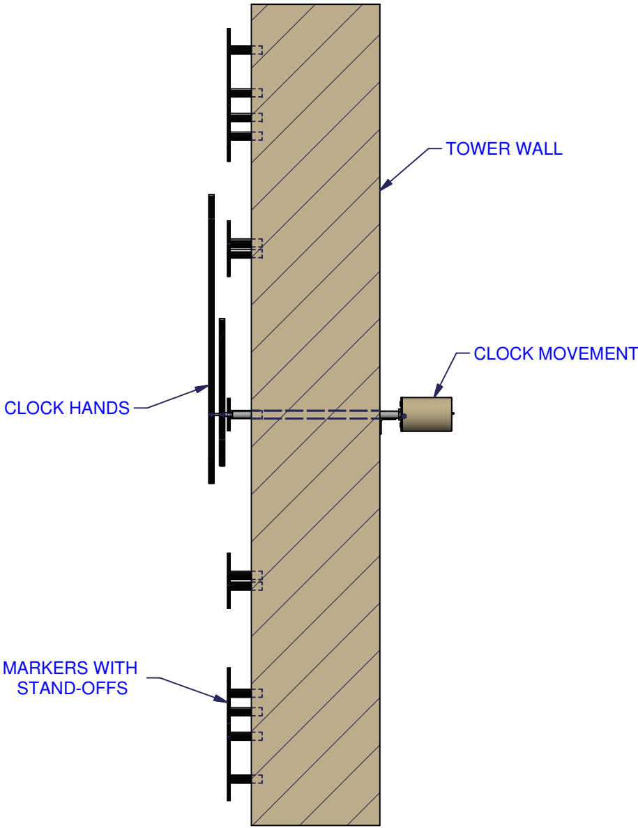
SECTION B-B
